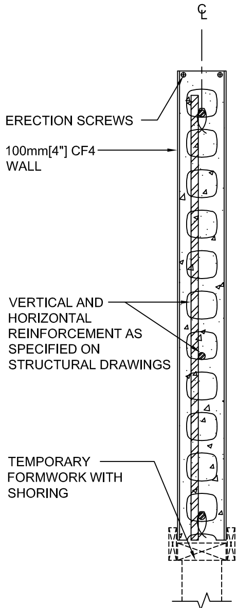
LINTEL OVER 450mm[1'-6"]
