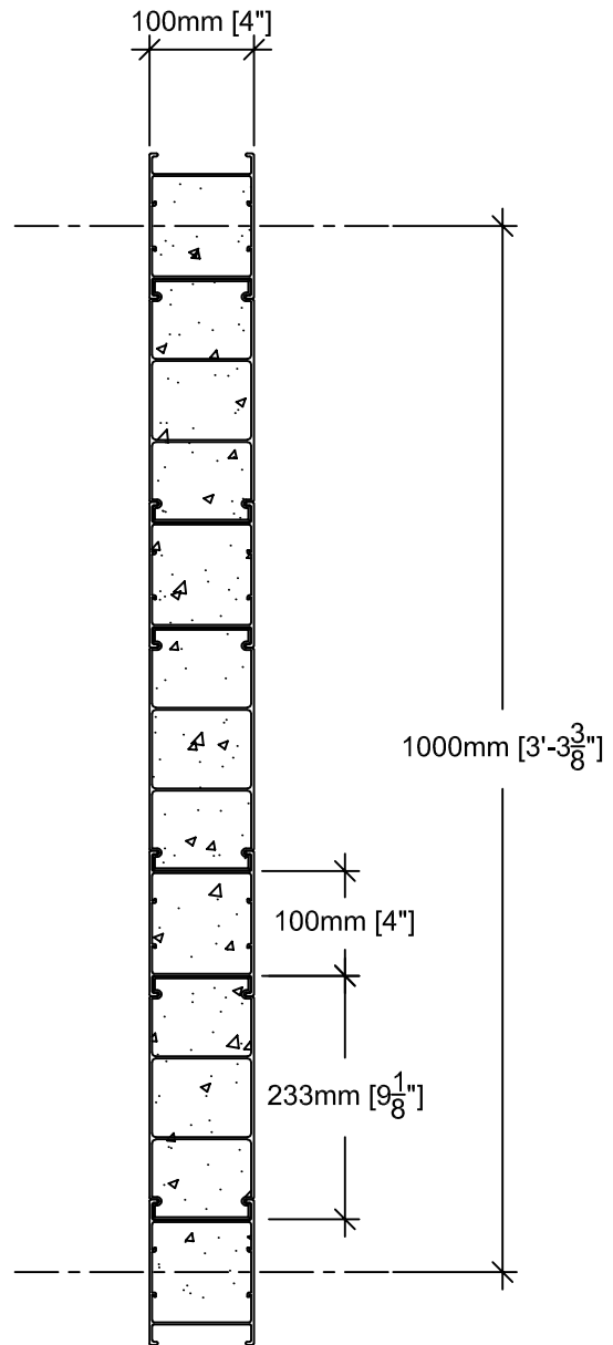
PLAN
