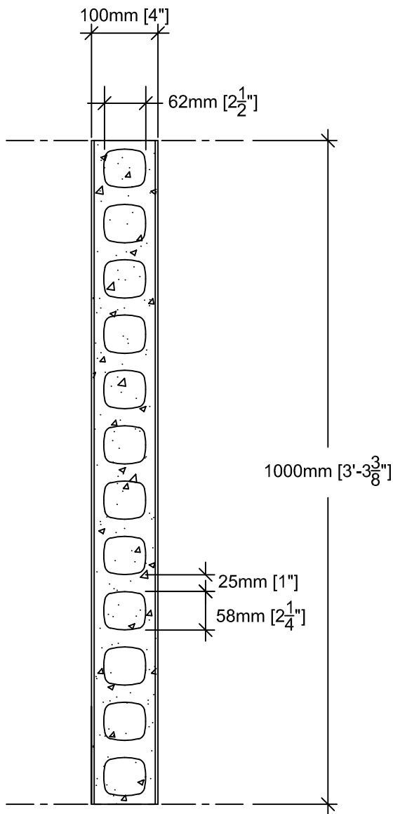
SECTION
