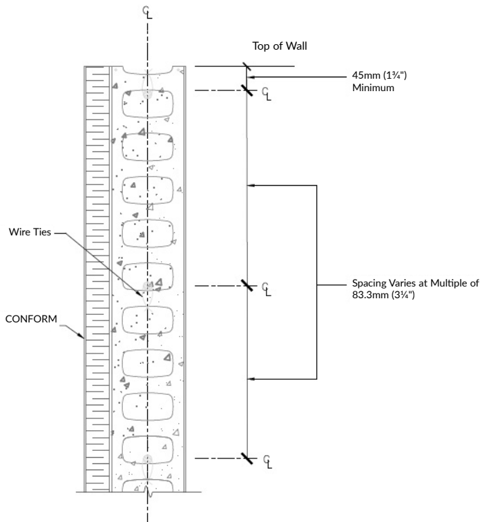
FIG. 2.3 HORIZONTAL REINFORCING BARS
