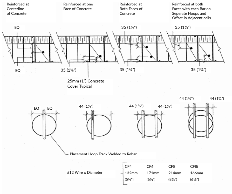
FIG. 2.3 HORIZONTAL REINFORCING BARS
