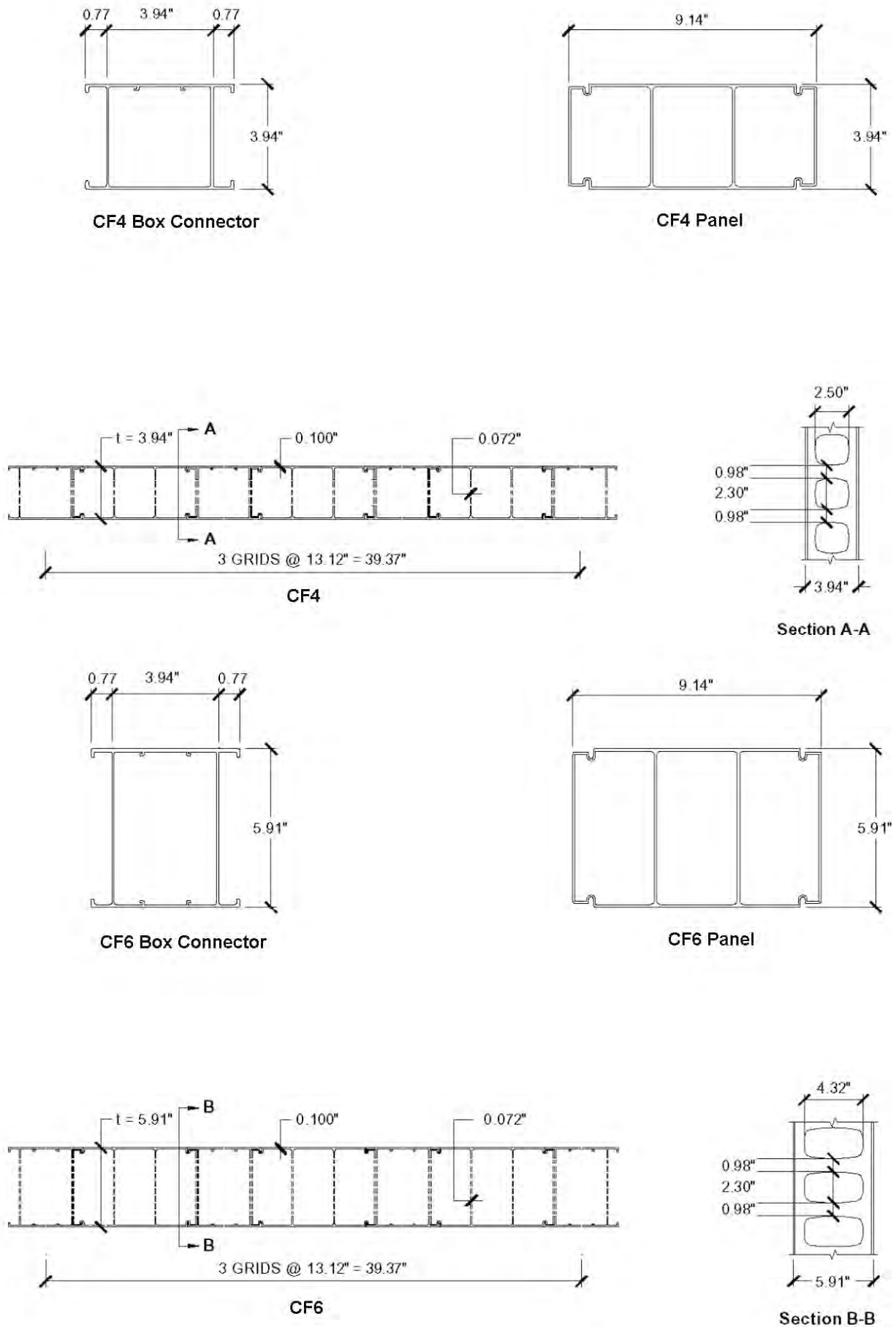
FIGURE 1—CF4 AND CF6 BOX CONNECTORS AND PANELS
