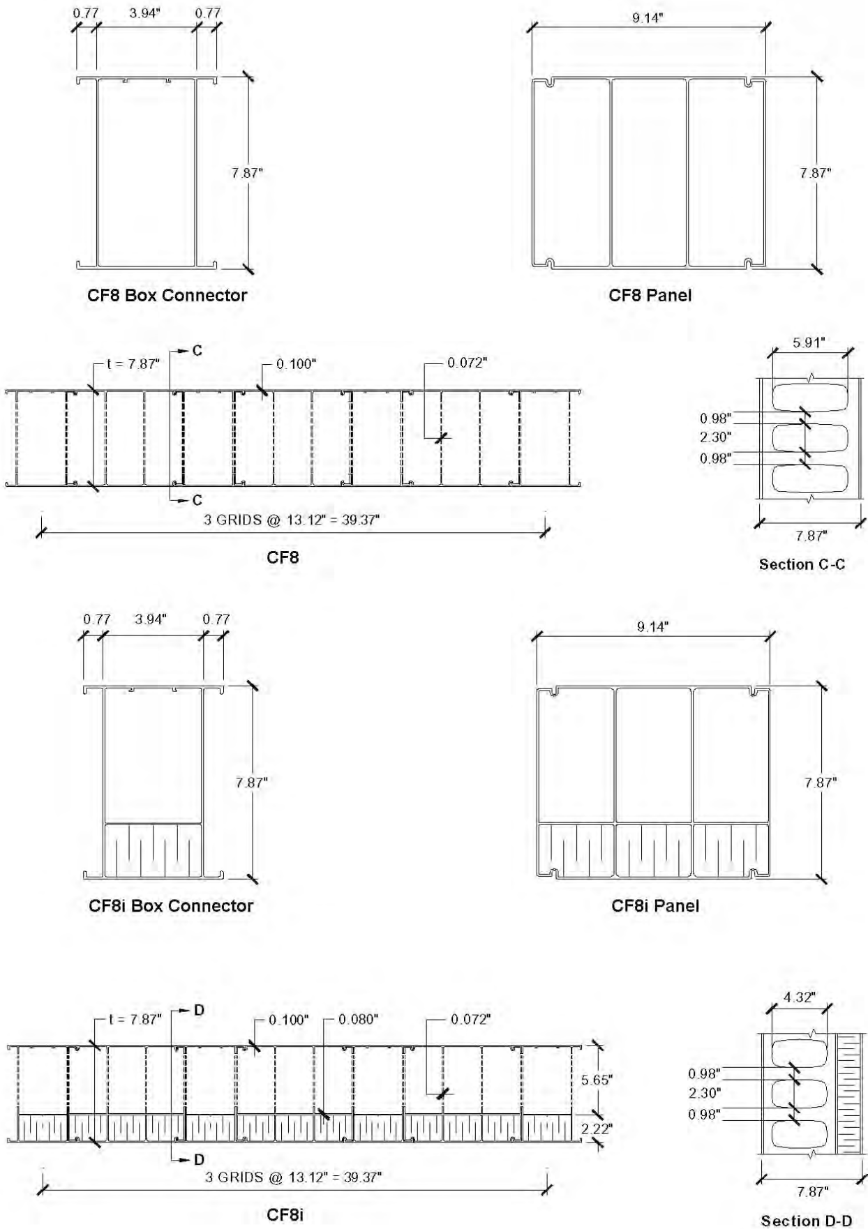
FIGURE 2—CF8 AND CF8i BOX CONNECTORS AND PANELS
