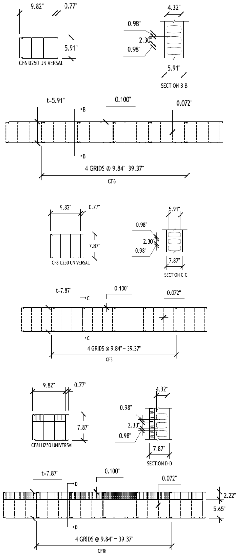
FIGURE 3—CF6, CF8 AND CF8i U250 UNIVERSAL PANELS
