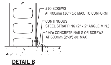
Fig B3-3b Single Steel Bracing with Strapping on One Side - Bottom Detail
