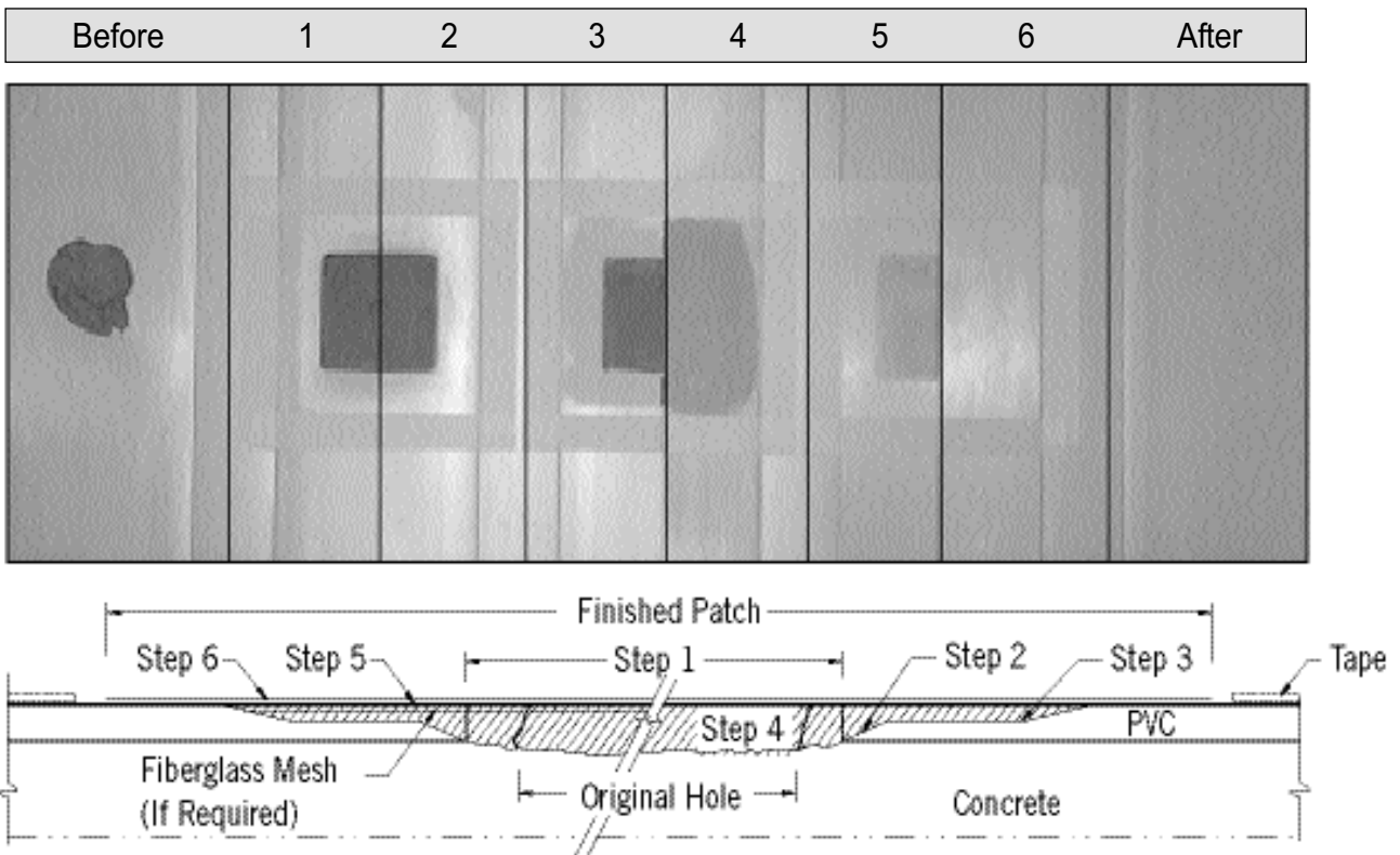
Figure 14.1: Repairing Surface Damage - Patching Holes
