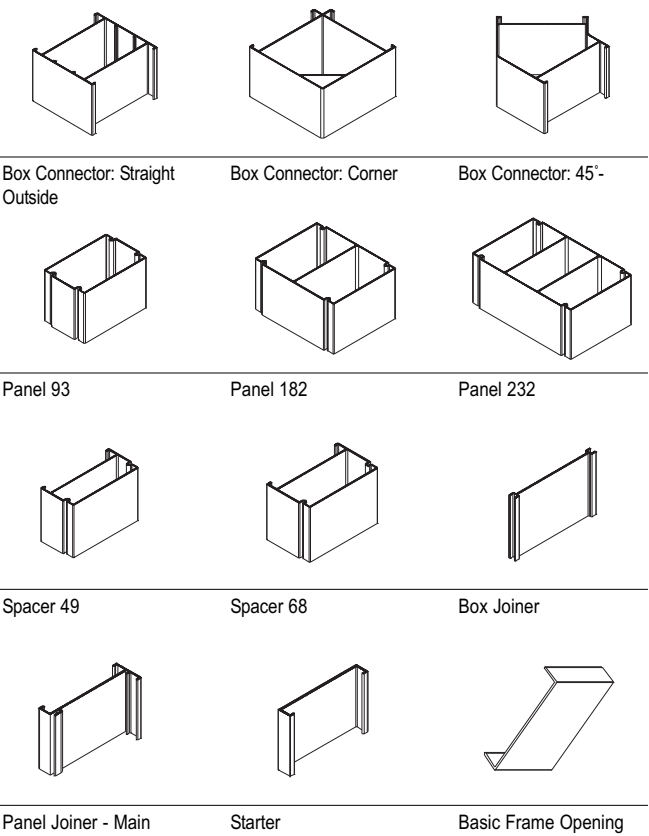
Fig 3.2 CF6 Components
