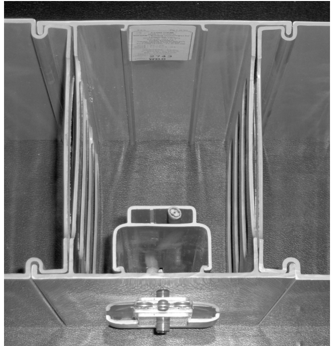
7.7c CONFORM Service Channel
