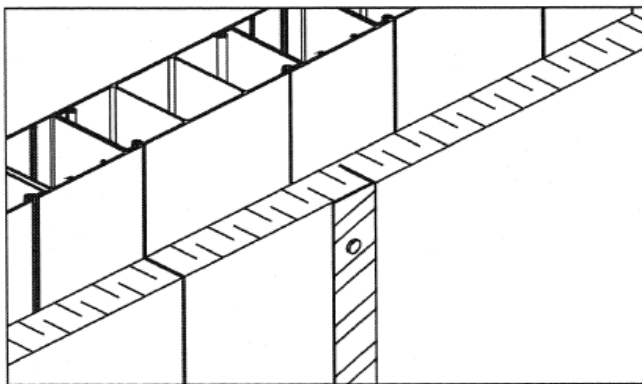
Figure 15.4: L or Angle Method
