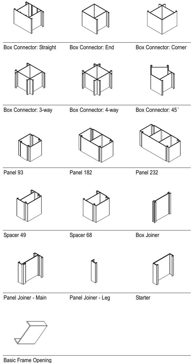
Fig 3.1 CF4 Components
