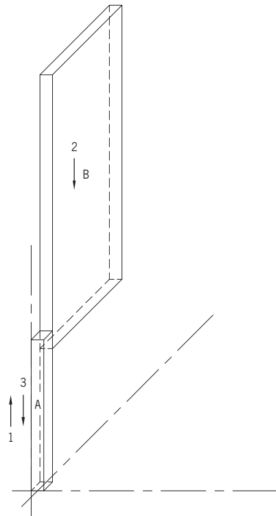
9.3b Erection Step 1
