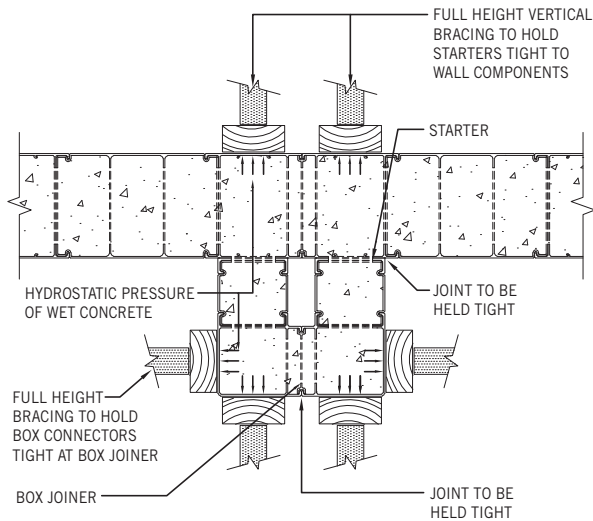
Fig B7-1 Pilaster Bracing
