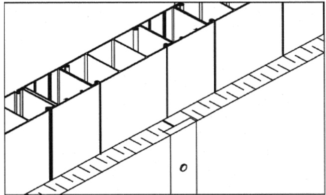
Figure 15.5: Wood Furring Strip Method
