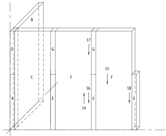
9.3e Erection Step 4
