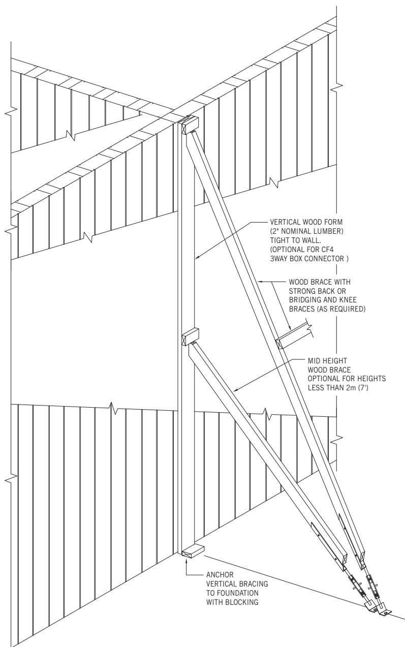
Fig B5-2 Vertical Tee Intersection Bracing
