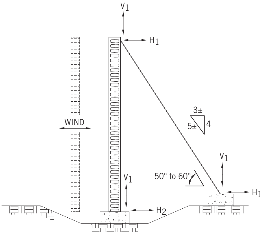
Fig B2 Bracing Force Diagram
