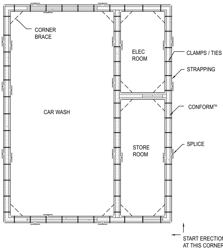
Fig B8-3a Preliminary Bracing Layout
