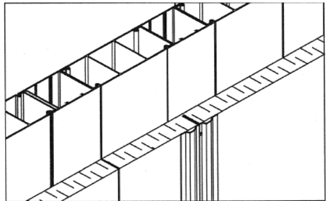
Figure 15.6: T-Strip Method
