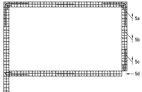
10.3d Corner Walls and Intersecting Walls
