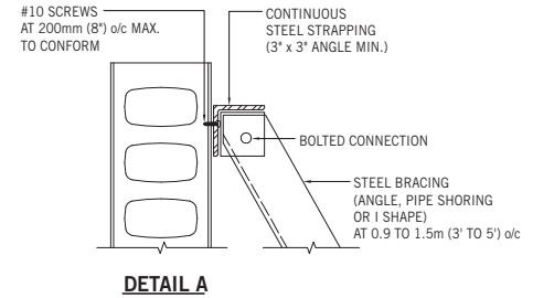
Fig B4-2a Double Steel Bracing with Strapping on One Side - Top and Mid-Height Detail
