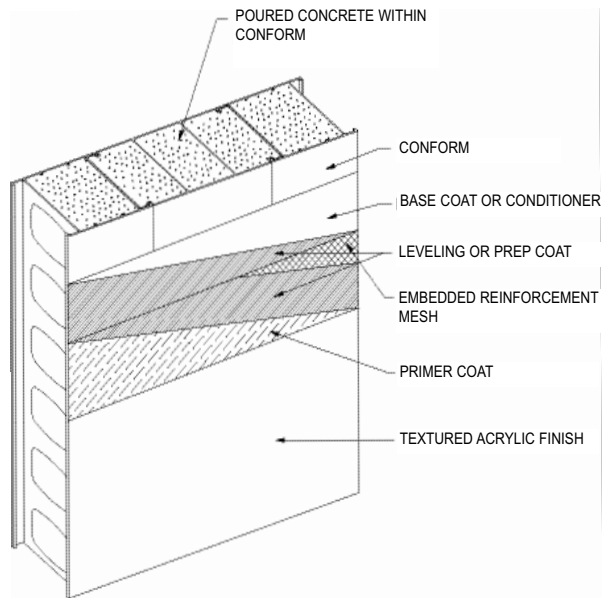
Figure 15.1: Stucco - Direct Apply Method
