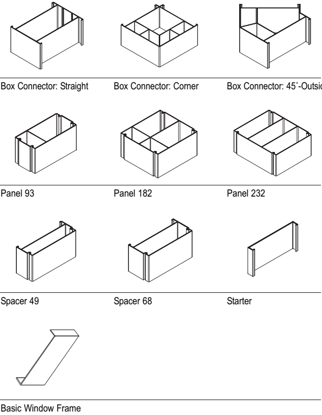
Fig 3.3 CF8 Components
