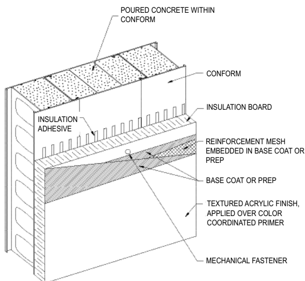
Figure 15.2: Stucco - EIFS System Method
