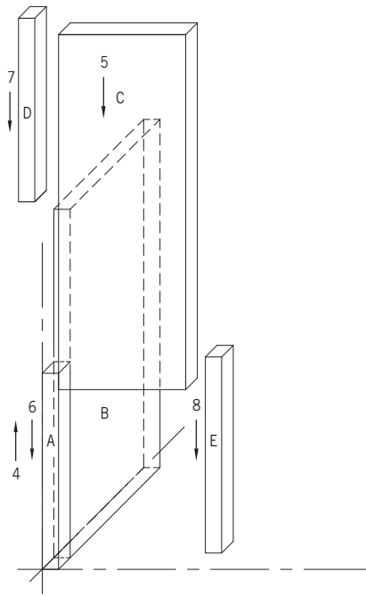
9.3c Erection Step 2
