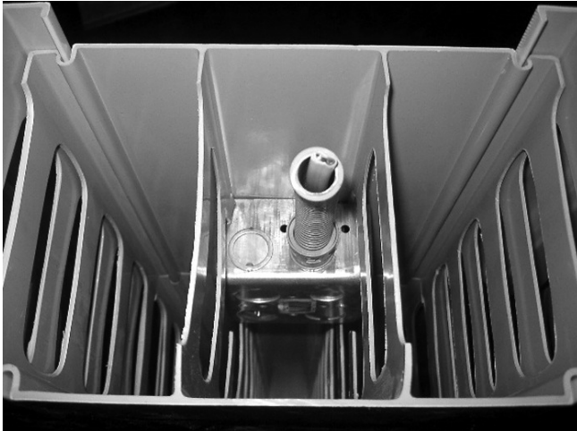
7.7a Electrical Box and Conduit
