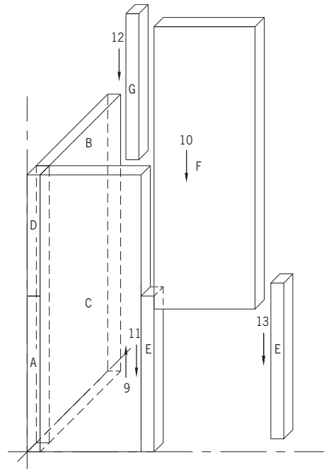
9.3d Erection Step 3
