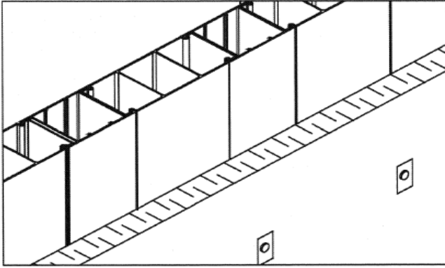
Figure 15.3: Plastic Washer Method
