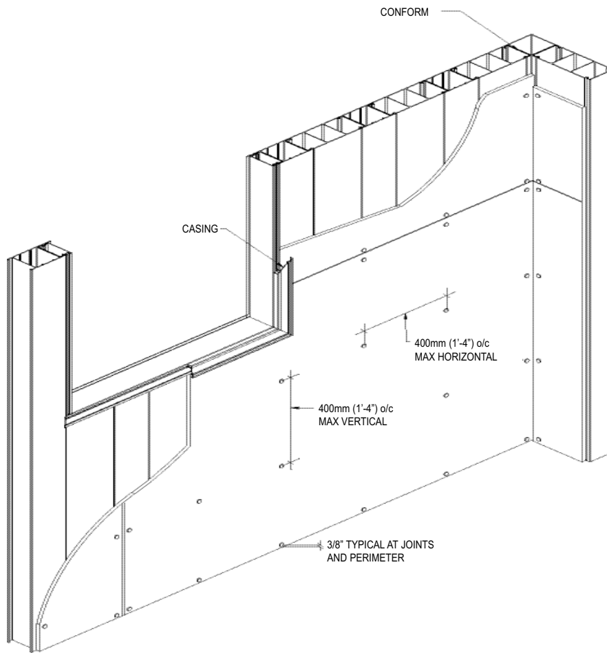
Figure 15.8: Gypsum Board
