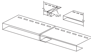
Figure 8 – J-Trim Overlap
