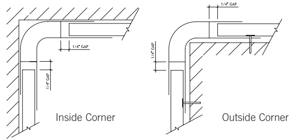
Figure 11 – Corner Trim
