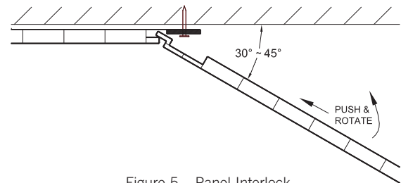
Figure 5 – Panel Interlock
