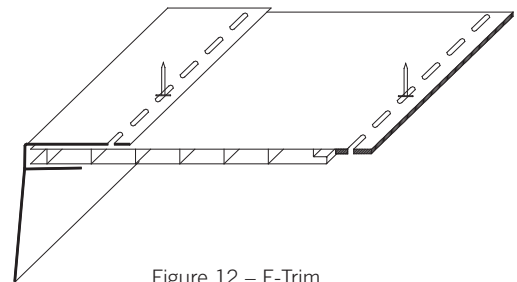
Figure 12 – F-Trim
