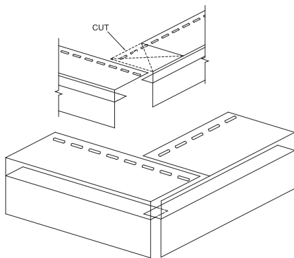
Figure 10 – F-Trim Corner
