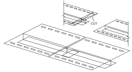
Figure 9 – H-Trim Overlap
